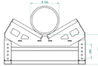
UAPR-1000G-400 Full Assembly
