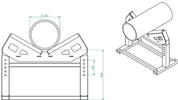
UAPR-1000G-650 Full Assembly
