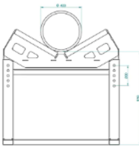
UAPR-1000G-900 Full Assembly
