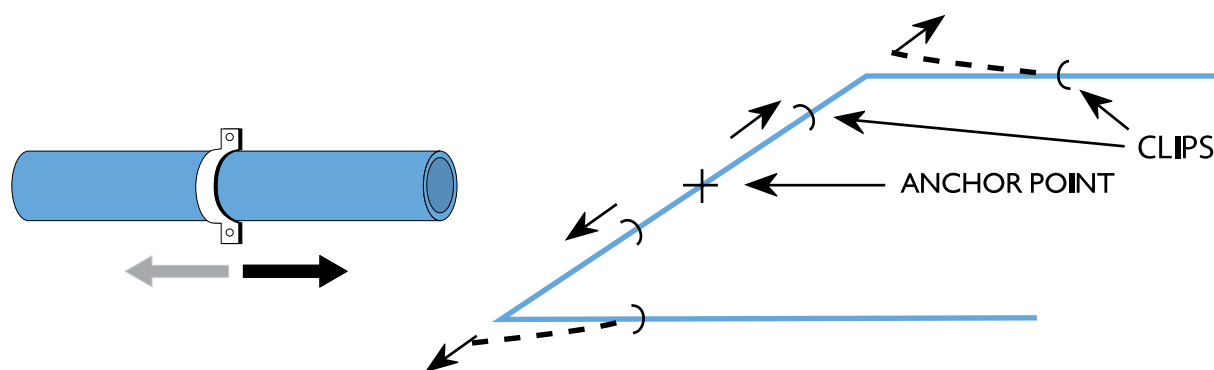
Free axial movement of pipework should be allowed with any form of support. Pipework should be able to move longitudinally without conflicting with elbows, tees, etc.
