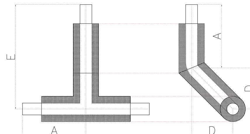
CROSSOVER TEE
