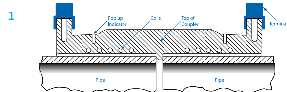
Pipe positioned in coupler prior to energising coil.
