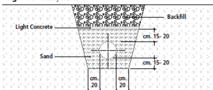
Figure 2 Heavy Traffic
