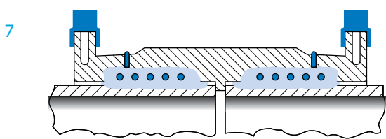
Melt pressure reaches optimum value at end of energising cycle. The pop up indicator appears to show fusion is complete.
