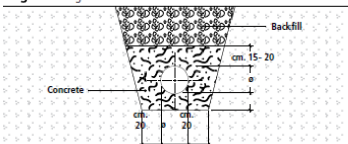
Figure 3 Rigid Installation
