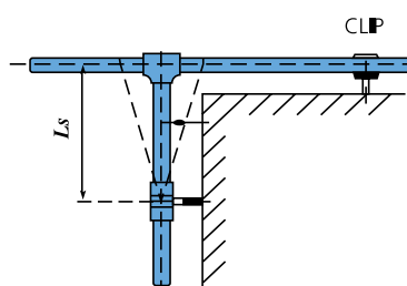
Clip placement for external corner
