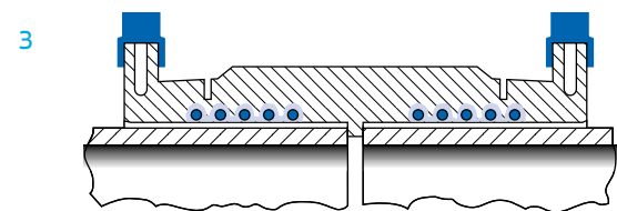
Material surrounding coil starts to melt.
