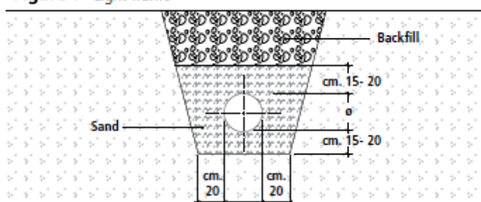
Figure 3 Rigid Installation
