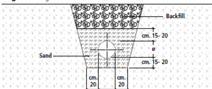
Figure 1 Light Traffic
